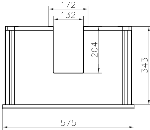
PLAN ELEVATION
