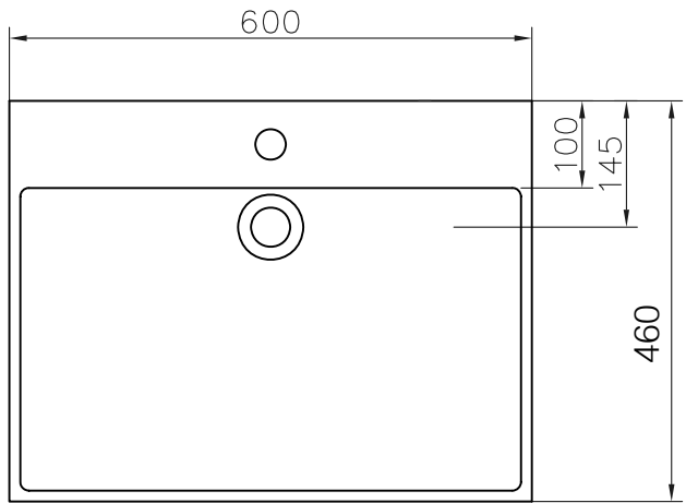
PLAN ELEVATION
